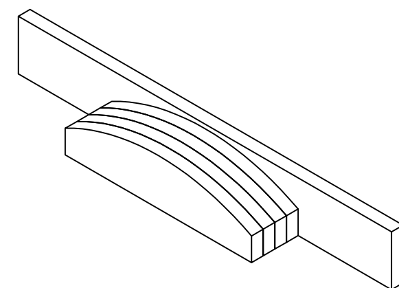
7 RIBBON LAYOUT JIG - ISO Scale: NTS
