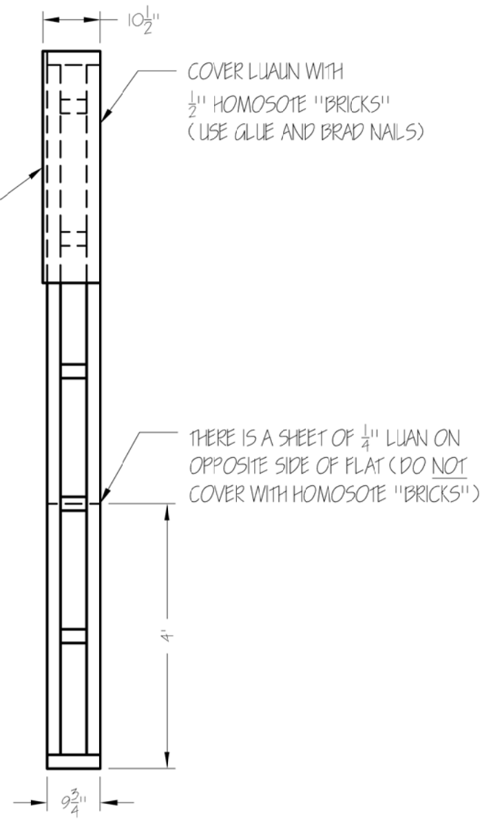
BANKS'S CHIMNEY WALL 1 SKIN - FRONT ELEVATION
