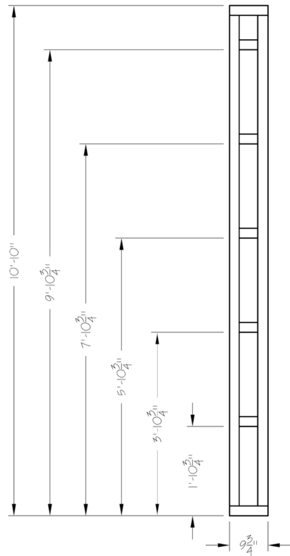
BANKS'S CHIMNEY WALL 1 FRAME - FRONT ELEVATION
