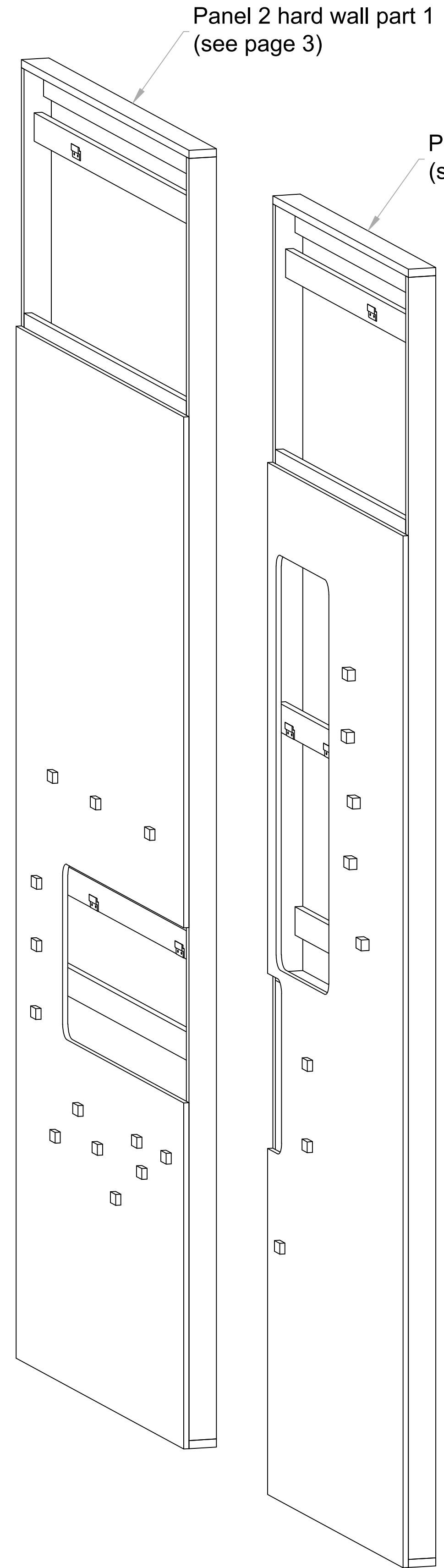
1 FRONT ISO - EXPLODED Scale: NTS
