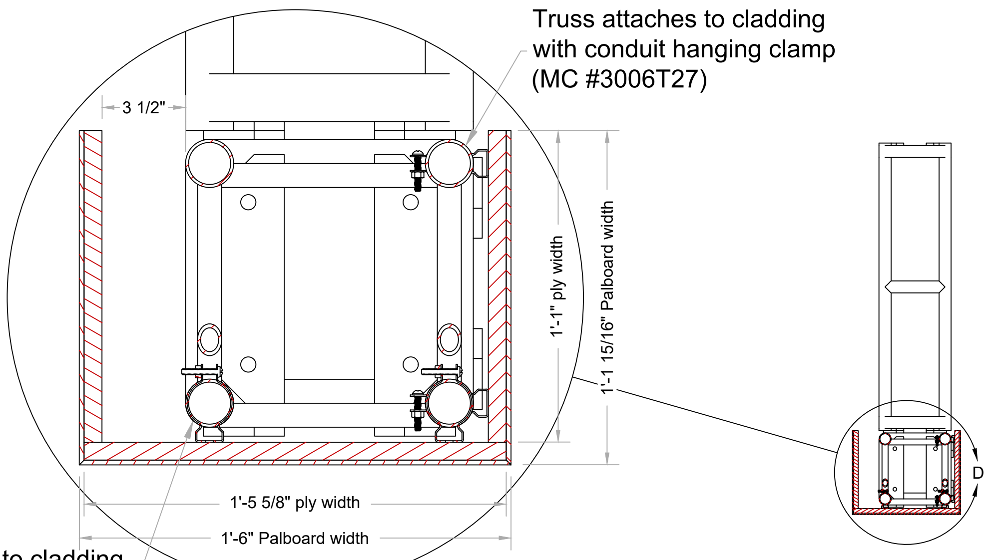
1 SECTION C-C SCALE 3/4" = 1'-0"
