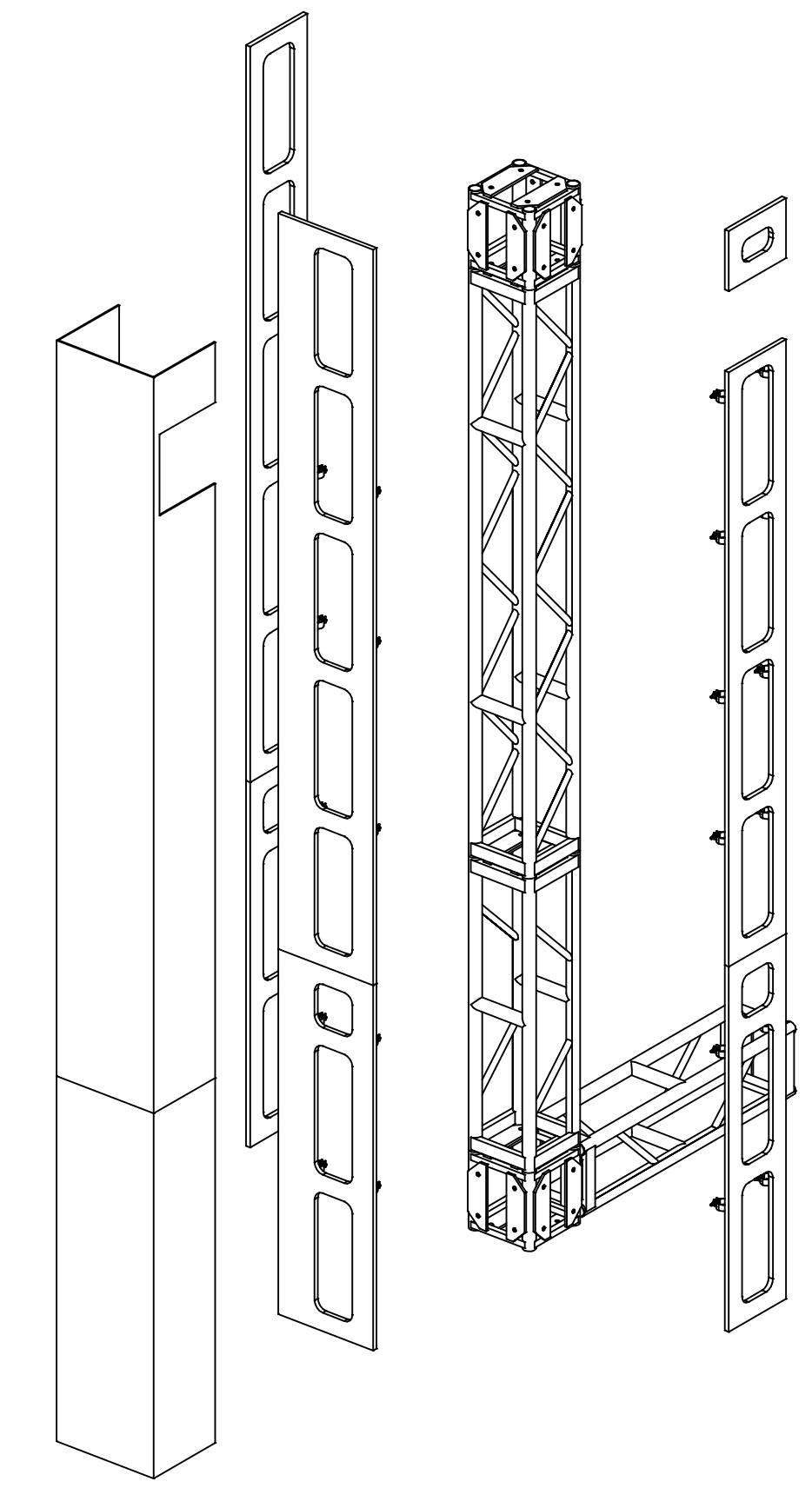
7 SEPARATED ISO VIEW Scale: NTS
