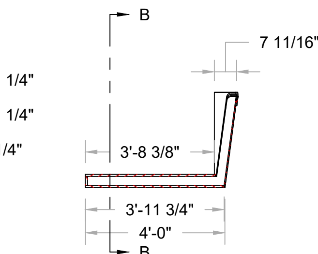
3 SECTION A-A SCALE 3/8" = 1'-0"
