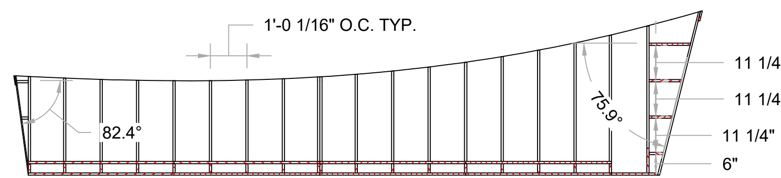
4 SECTION B-B SCALE 3/8" = 1'-0"
