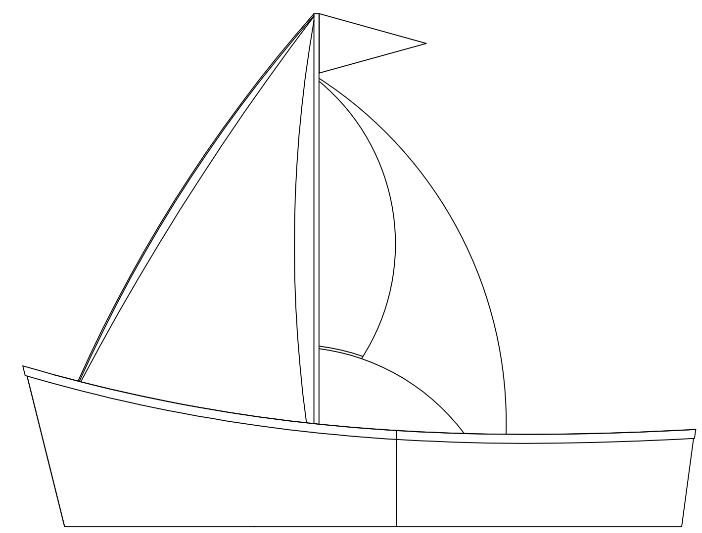
5 BOAT AND SAIL - FRONT VIEW Scale: 3/8" = 1'-0"
