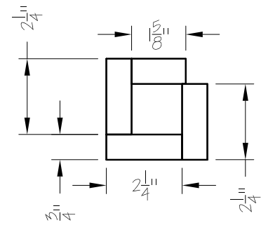
4 103 UPSTAGE UPRIGHTS - TOP VIEW 3/4" = 1'-0" RIP TO SIZE FROM 1X MATERIAL BUILD TWO (2); REVERSE AND REPEAT
