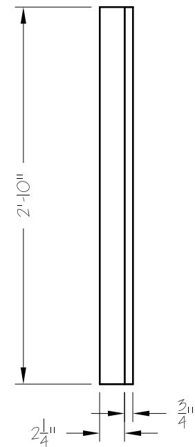
5 103 UPSTAGE UPRIGHTS - FRONT VIEW 1/2" = 1'-0" RIP TO SIZE FROM 1X MATERIAL BUILD TWO (2); REVERSE AND REPEAT
