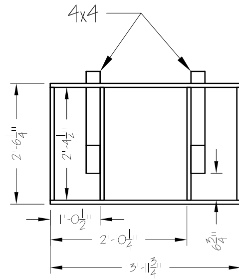
2 103 2 GENTS BALCONY - FRAME AND DIAGONALS 1/2" = 1'-0" FRAME IS 1X2 STEEL TUBE WELD ALL JOINTS GRIND DOWN WELDS ON TOP AND SIDES USE 3/8" X 5" BOLTS TO CONNECT 4X4s TO FRAME
