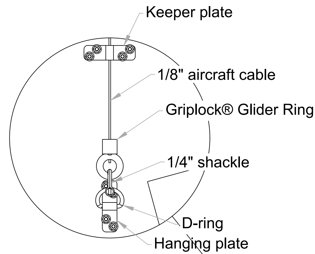
DETAIL P SCALE 3" = 1'-0"
