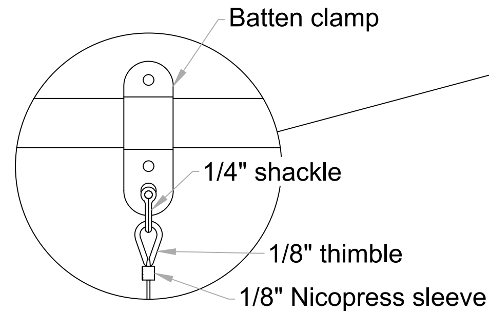
DETAIL O SCALE 3" = 1'-0"
